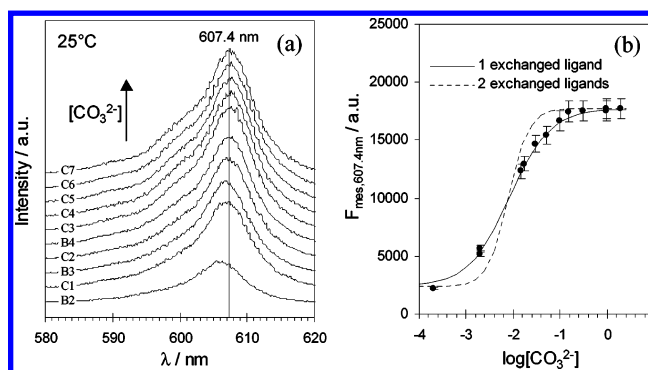
Figure 1. [CO 3 2- ] influence on the speciation of Cm(III) in bicarbonate and carbonate solutions at I = 3 \text{ M} and 25 °C. (a) Fluorescence spectra corresponding to the solutions whose labels are indicated on the graphic, referring to Table 1. (b) Fluorescence intensities at 607.4 nm, the wavelength of the maximum intensity for Cm(CO 3 ) 3 3- , over \log[\text{CO}_3^{2-}] . The curves were adjusted considering the exchange of 1 (solid line) and 2 (dashed line) ligands and gave evidence of the exchange of one CO 3 2- in the dissociation reaction.
