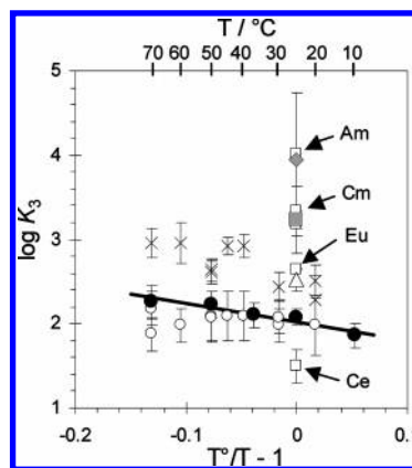
Figure 3. Comparison of \log K_3 values at various temperatures for Am(III) and Ln(III). K_3 values were corrected to I = 3 \text{ M NaClO}_4 with the SIT formula (eqs 4 and 5). TRLFS data for Cm(III) from this work (●) (Table 2); Am(III) solubility data obtained in 3 M \text{NaClO}_4 10 (△), in 4 M \text{NaCl} media 12 (×), and our reinterpretation (○); selected constants for Am(III) 5 (◆) and for Am/Cm(III) 15 (■); literature data for Am(III), 11 Cm(III), 23,24 Ce(III), 9 and Eu 44 (□) as indicated on the graphic.
