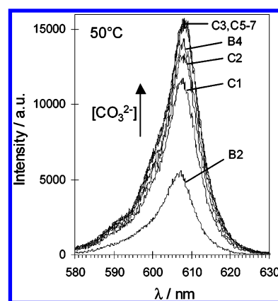
Figure 4. Influence of [\text{CO}_3^{2-}] on the fluorescence spectra measured at 50 °C. The solution labels are indicated on the graphic, referring to Table 2.
